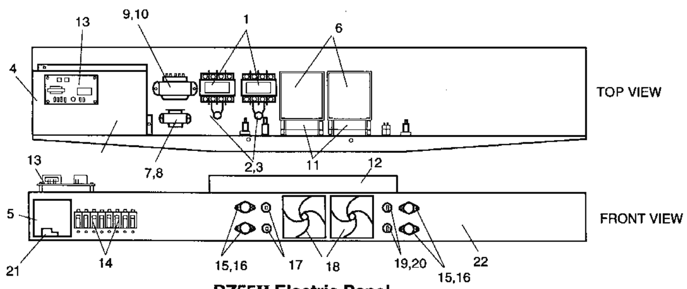
DZ55II Electric Panel
