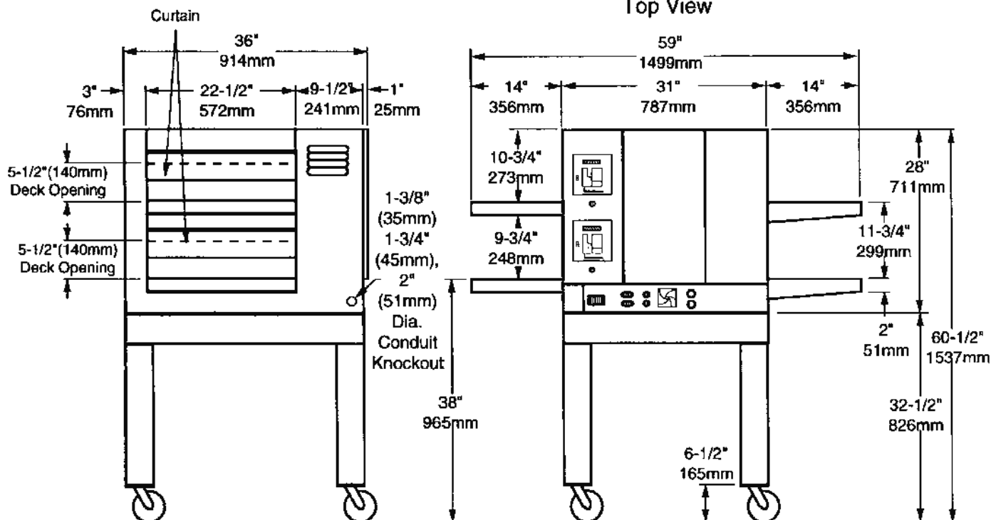
End View
