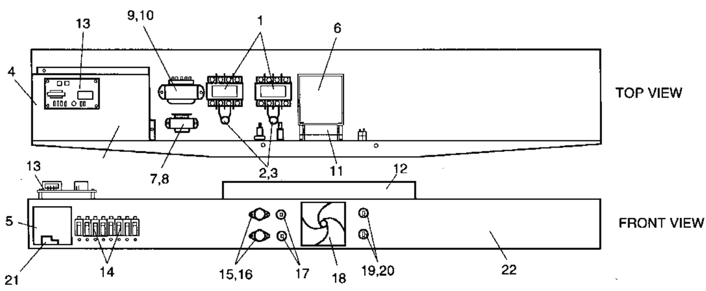
DZ55 Electric Panel
