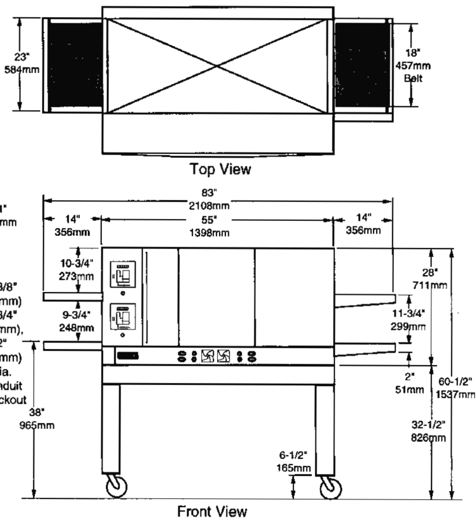
Model DZ55II Single Oven on Base with Two MenuSelect Controls
