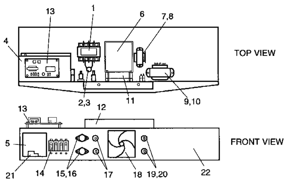
DZ33II and DZ33 Electric Panel
