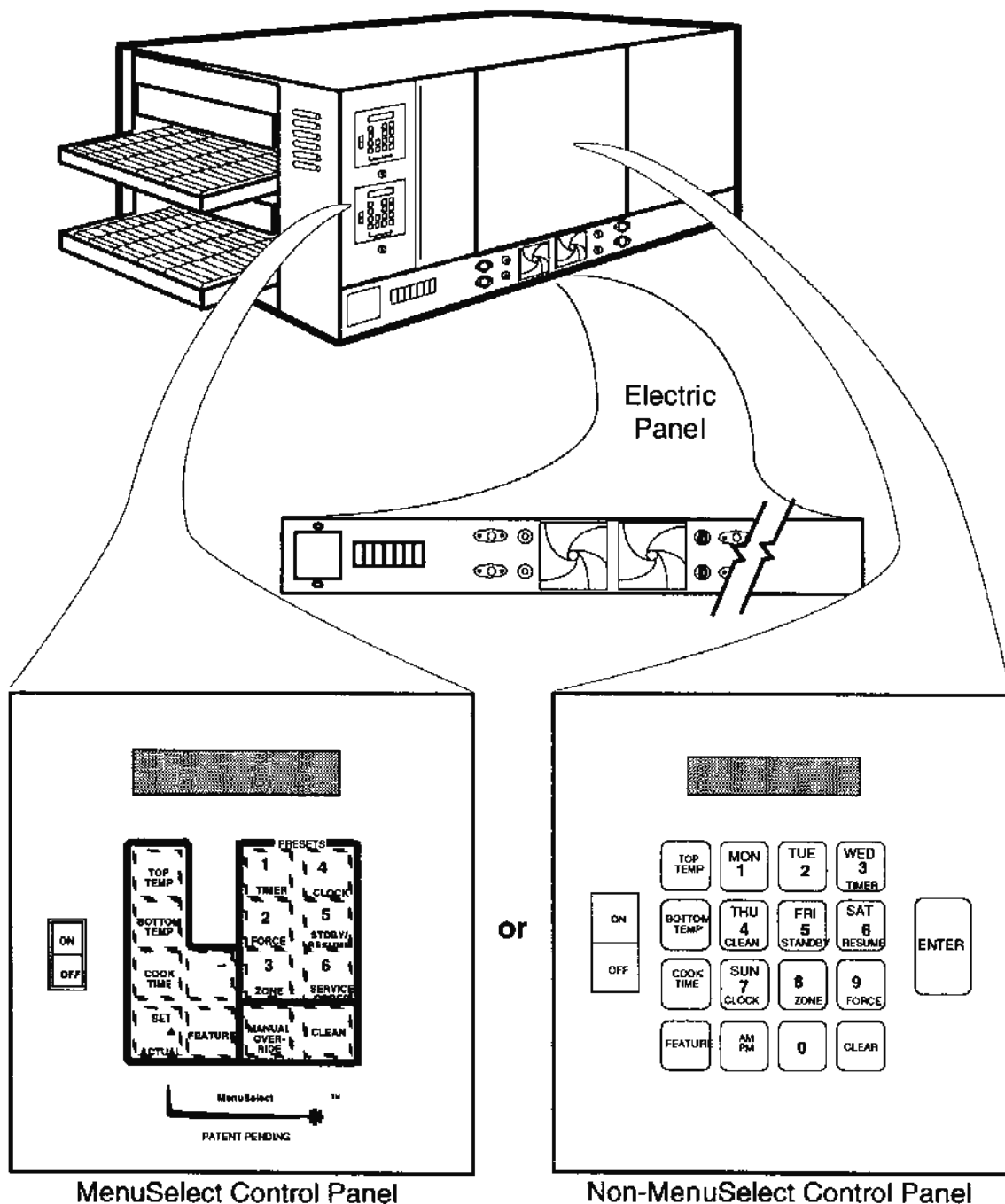
Figure 3-1 Operating Controls
