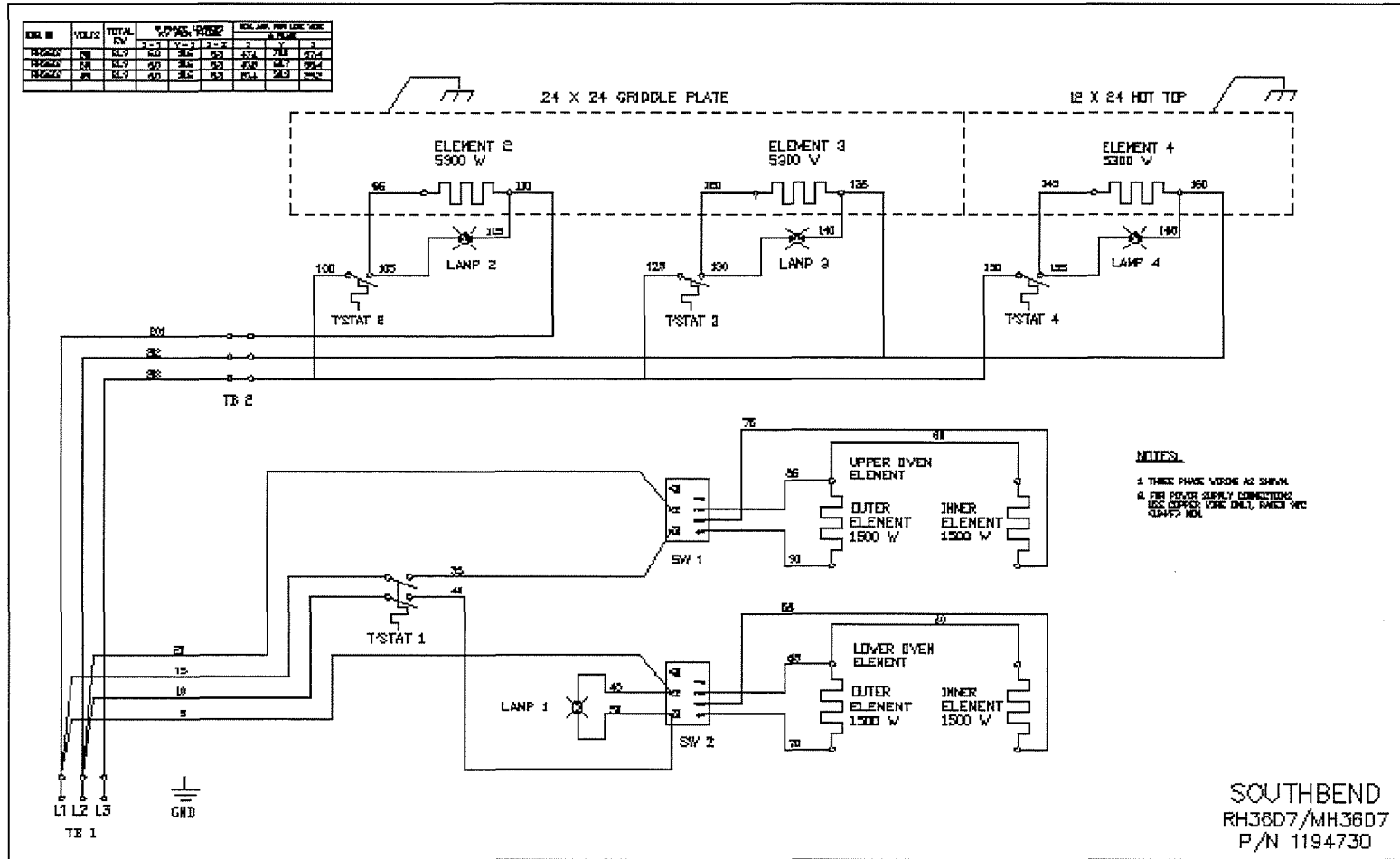
SE36D-TTH WIRING DIAGRAM 208/240V
