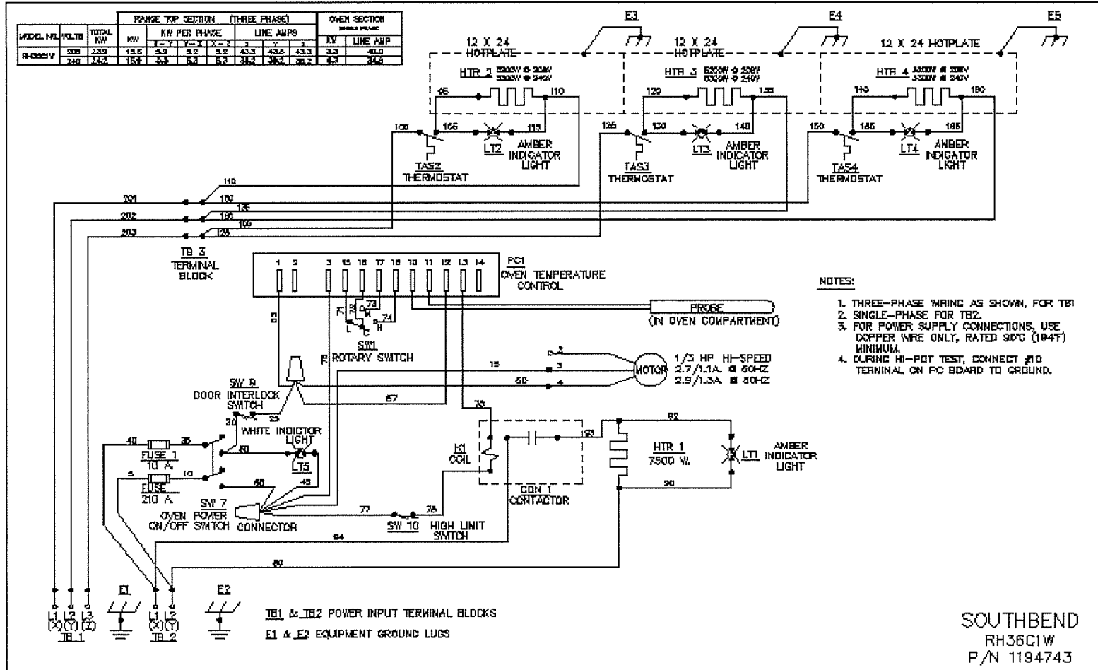
RH36C1W WIRING DIAGRAM 208/240V
