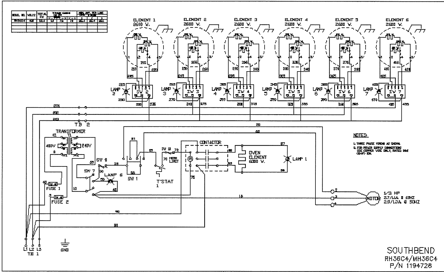
SE36A-BBB WIRING DIAGRAM 480V
