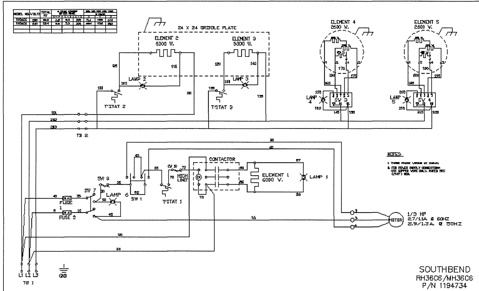
SE36A-TTB WIRING DIAGRAM 208/240V
