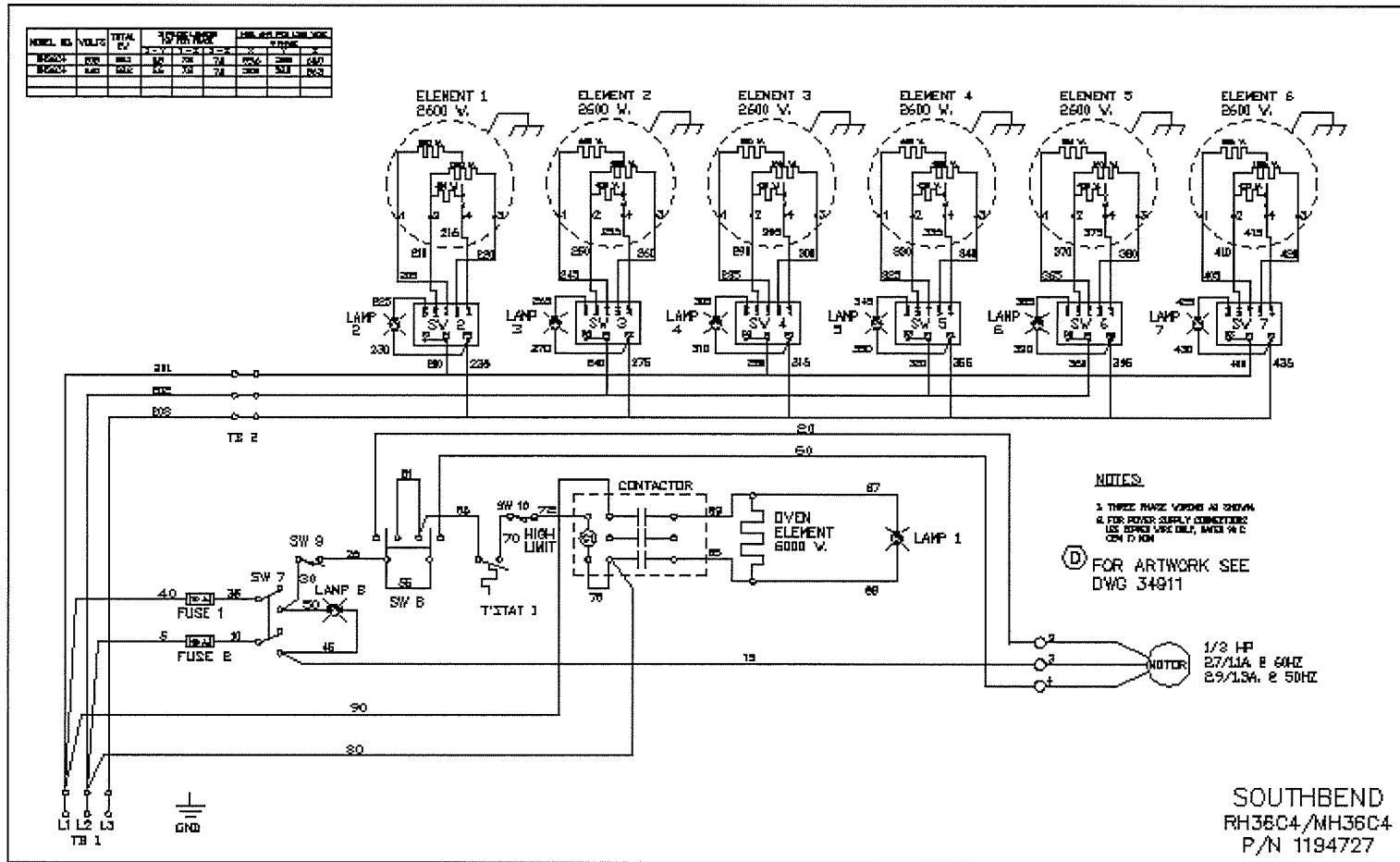
SE36A-BBB WIRING DIAGRAM 208/240V
