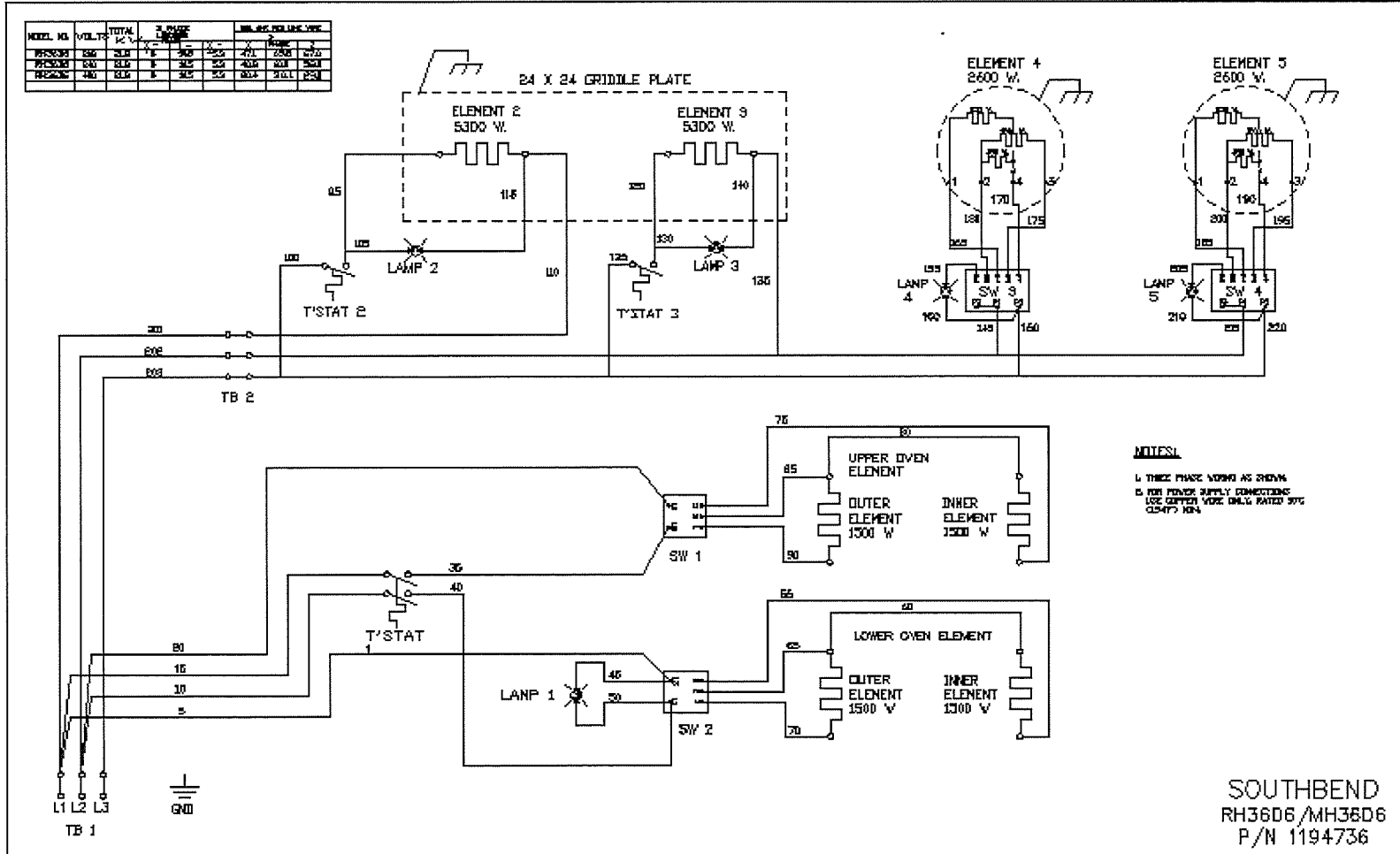
SE36D-TTT WIRING DIAGRAM 208/240V
