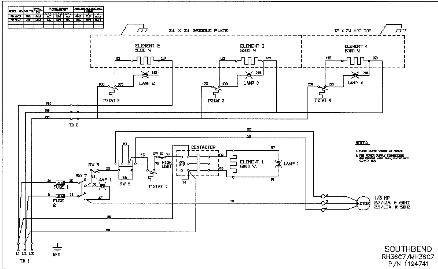
SE36A-TTH WIRING DIAGRAM 208/240V
