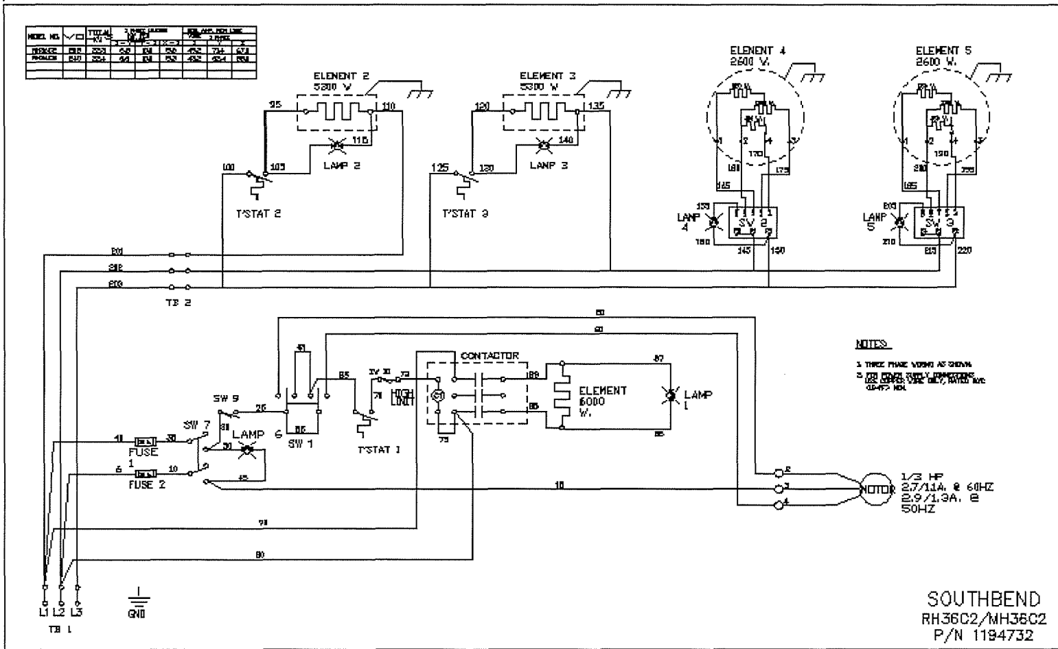
SE36A-HHB WIRING DIAGRAM 208/240V
