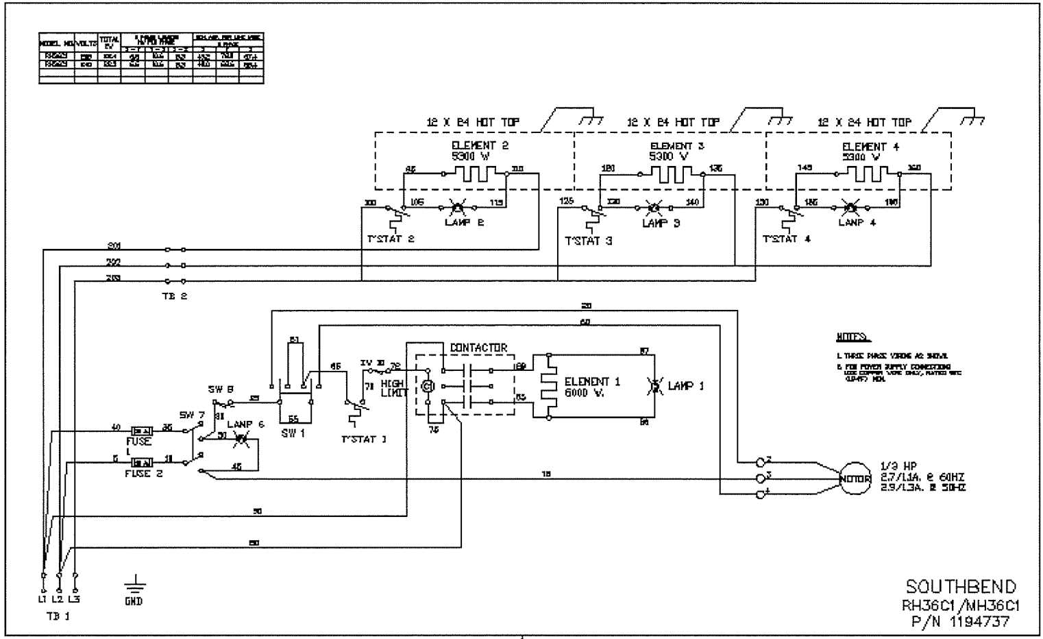
SE36A-HHH WIRING DIAGRAM 208/240V
