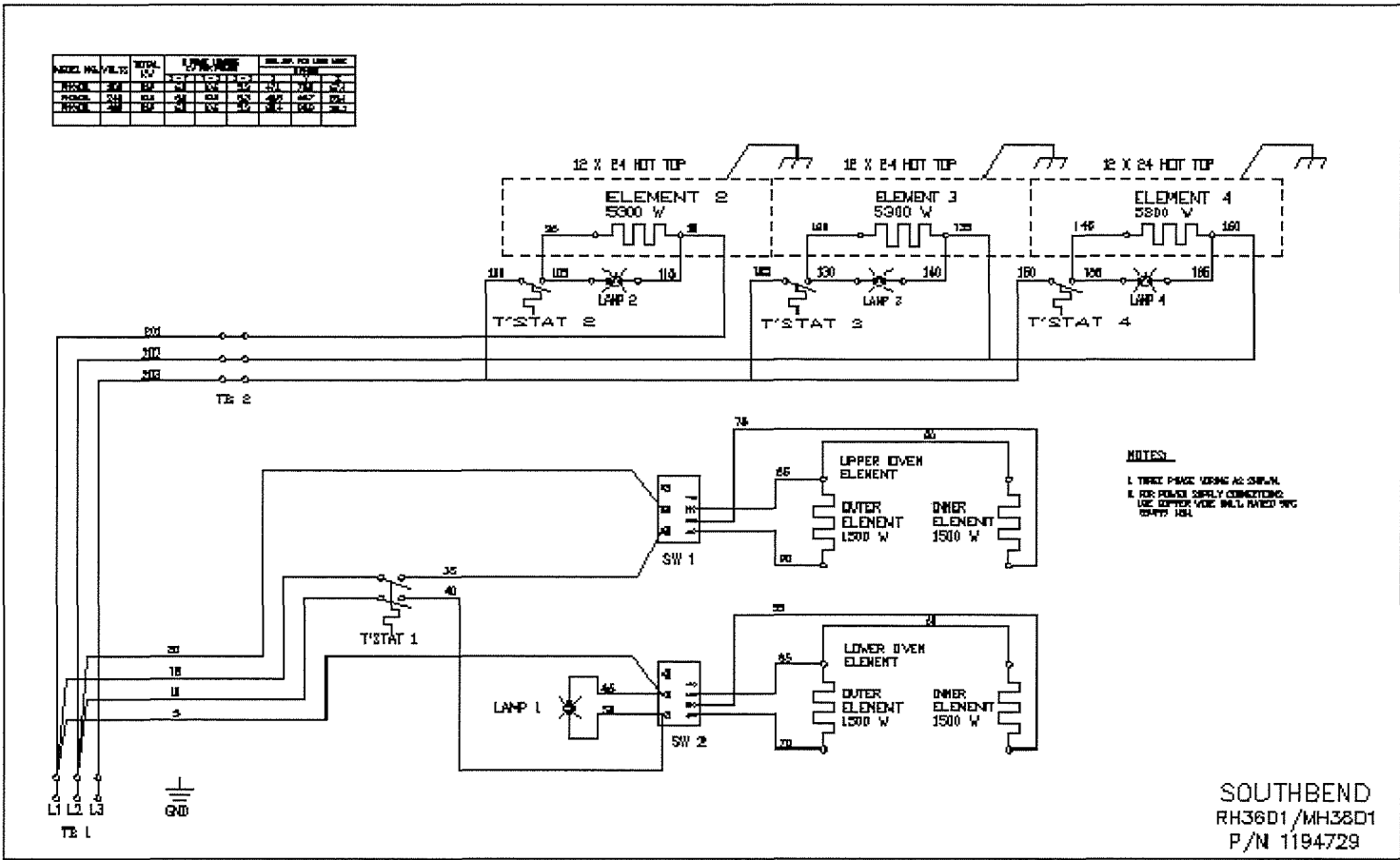
SE36D-HHH WIRING DIAGRAM 208/240V
