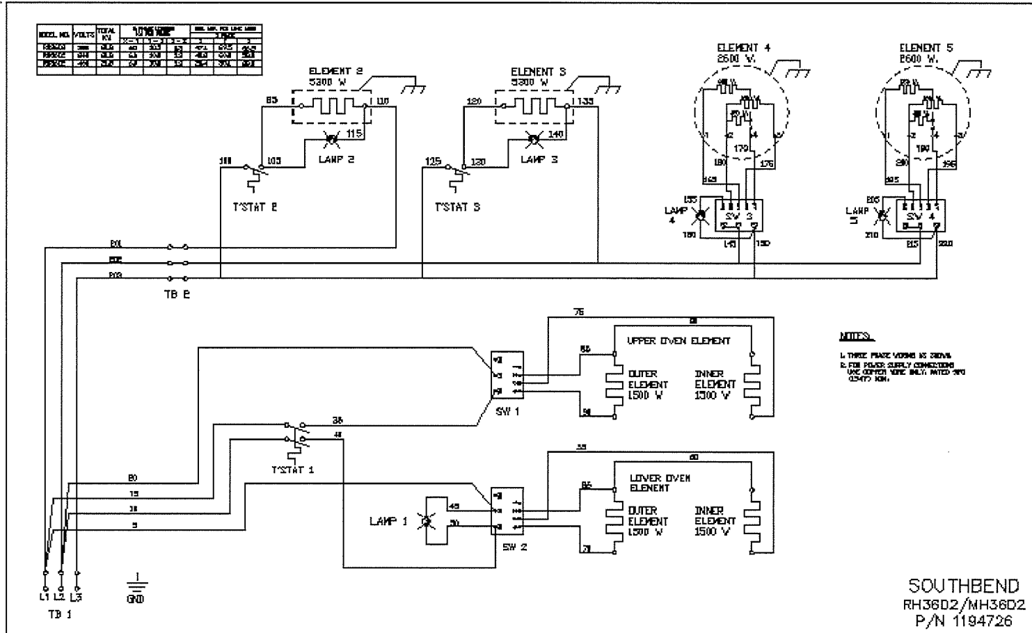
SE36D-HHB WIRING DIAGRAM 208/240V
