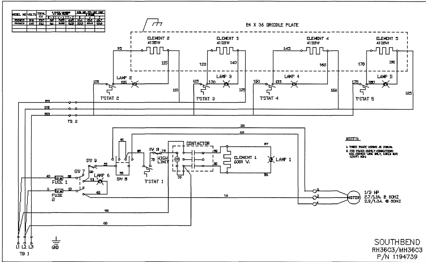
SE36A-TTT WIRING DIAGRAM 208/240V
