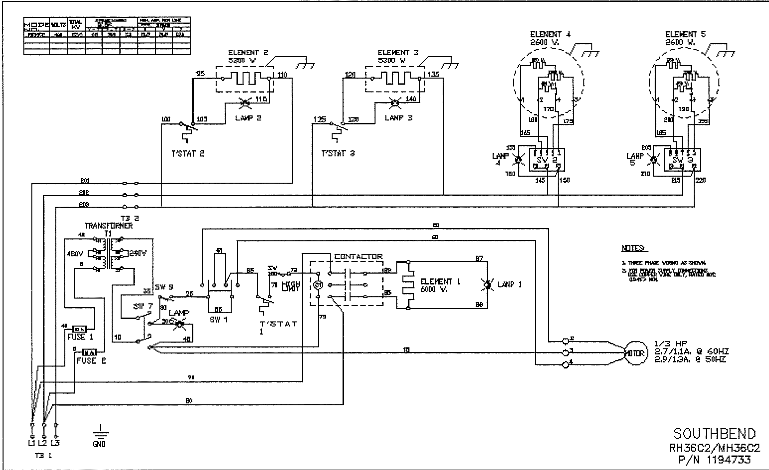
SE36A-HHB WIRING DIAGRAM 480V
