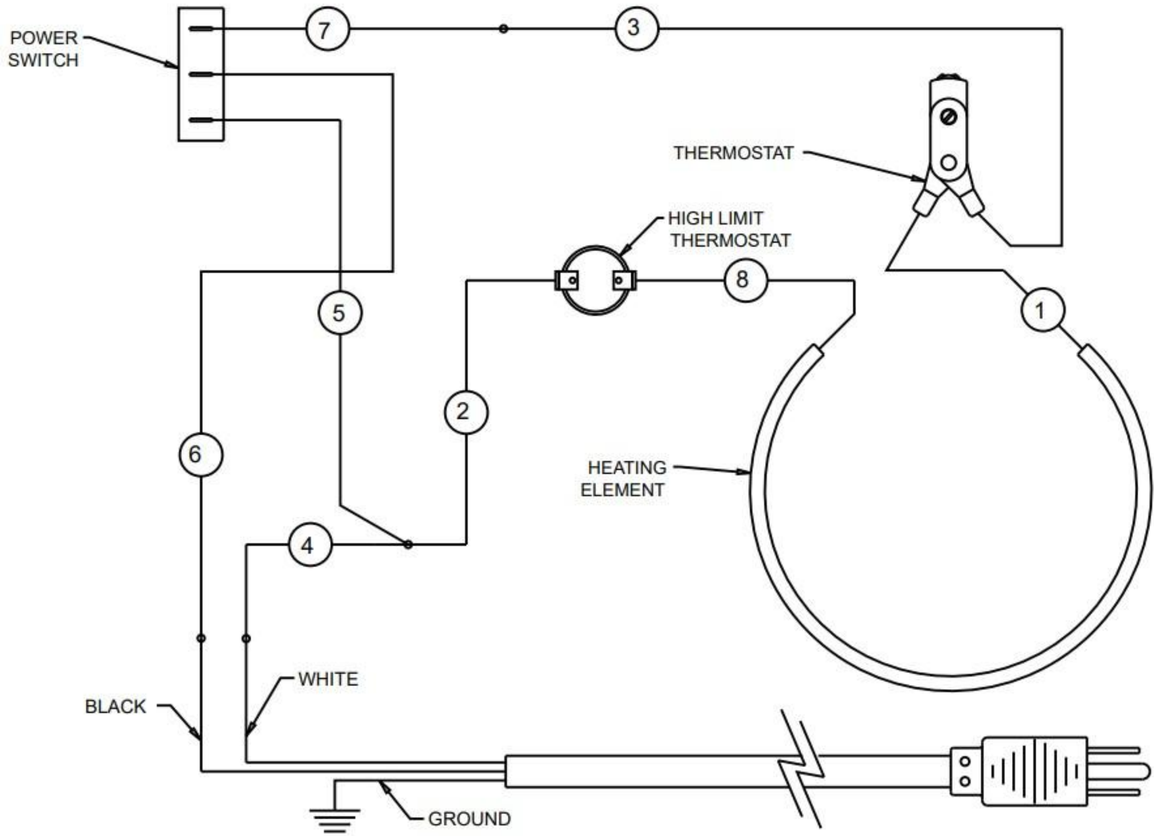
HDW-2 Wiring Diagram
